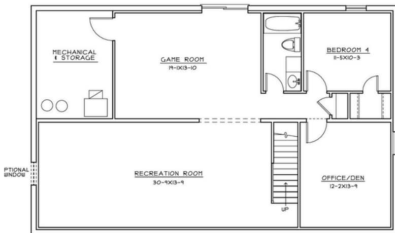
OPTIONAL FINISHED BASEMENT
